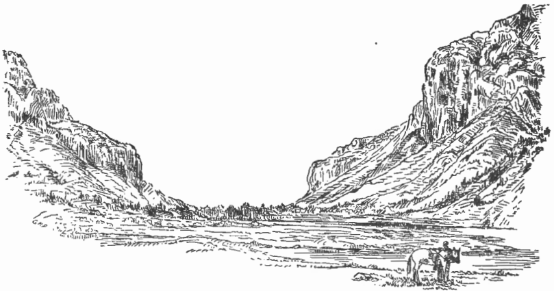
FIG. 9. DEVIL'S GAP VALLEY, LOOKING EAST.
